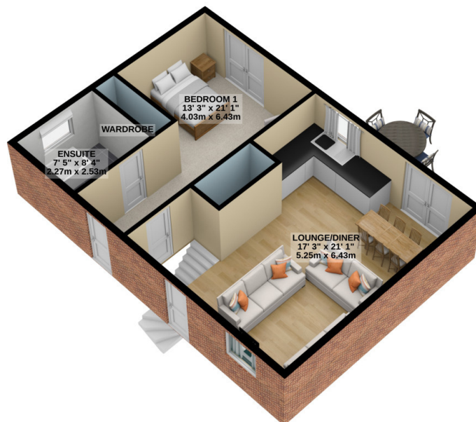
GROUND FLOOR 643 sq.ft. (59.7 sq.m.) approx.
